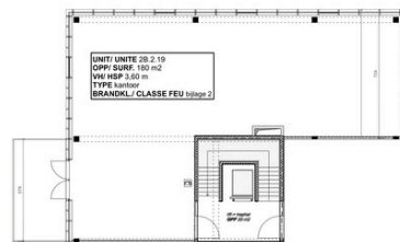
PLAN +1 - unit 2B.2.19
