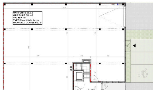
PLAN 0 - unit 2B.2.2
